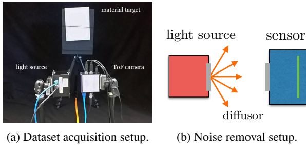
Figure 4: Illustrations of experimental setup.
