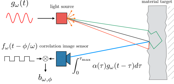
Figure 2: Temporal interaction of light and material. A correlation image sensor correlates the reference signal with a mixture of (a) direct surface reflection (black); (b) surface inter-reflection or multiple scattering inside surface volume (red); and (c) subsurface scattering (green). The camera observes a mixture of (a),(b) and (c), as indicated in blue.
