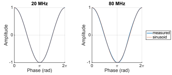
Figure 5: Our modulation signal \phi_{\omega}(t) at 20MHz and 80MHz.
